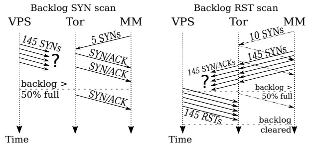
(a) SYN scan to infer whether SYN segments from VPS reach Tor. “MM” is our measurement machine. (b) RST scan to infer whether RST segments from VPS reach Tor. “MM” is our measurement machine.
